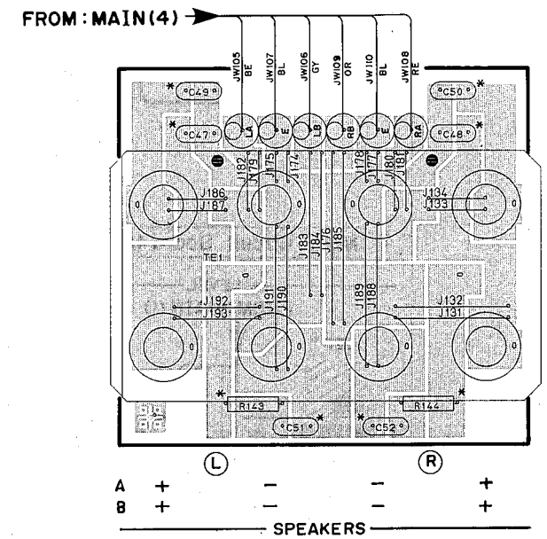
Main Circuit Board (5)
