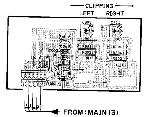
LED Circuit Board (1)
